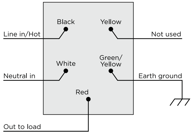
Figure 2. Single device location, with neutral connection (recommended)
