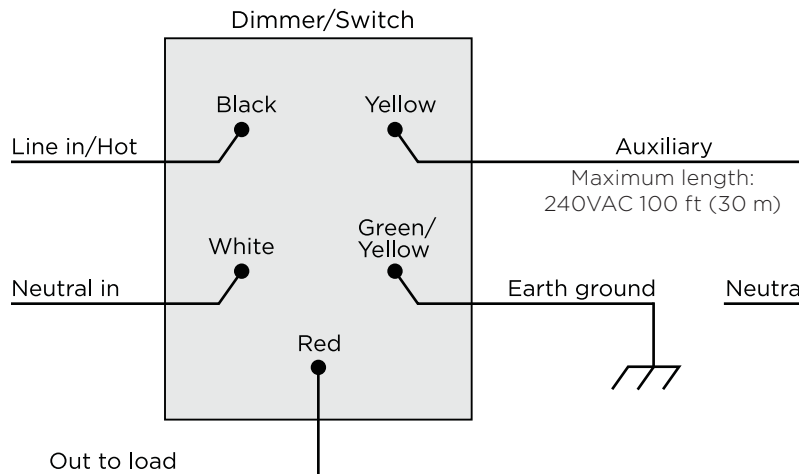
Figure 4. Multiple device location using Auxiliary Keypad, with neutral connection (recommended)
