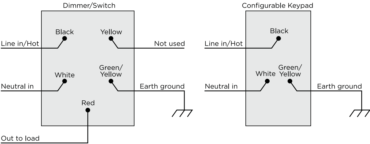
Figure 6. Multiple device location using Configurable Keypad, neutral required
